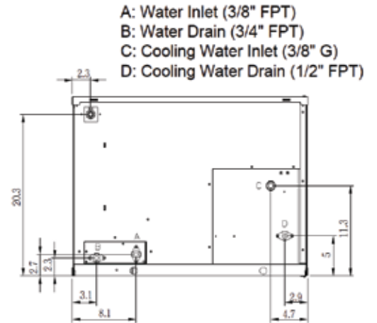
BACK VIEW
